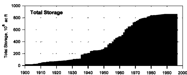
Figure 3. History of increasing total reservoir storage for the continental United States. Data from U.S. Army Corps of Engineers [1996].
